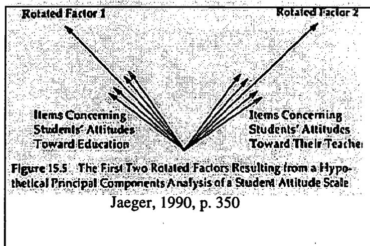
Figure 4. Rotated variables and factors.
